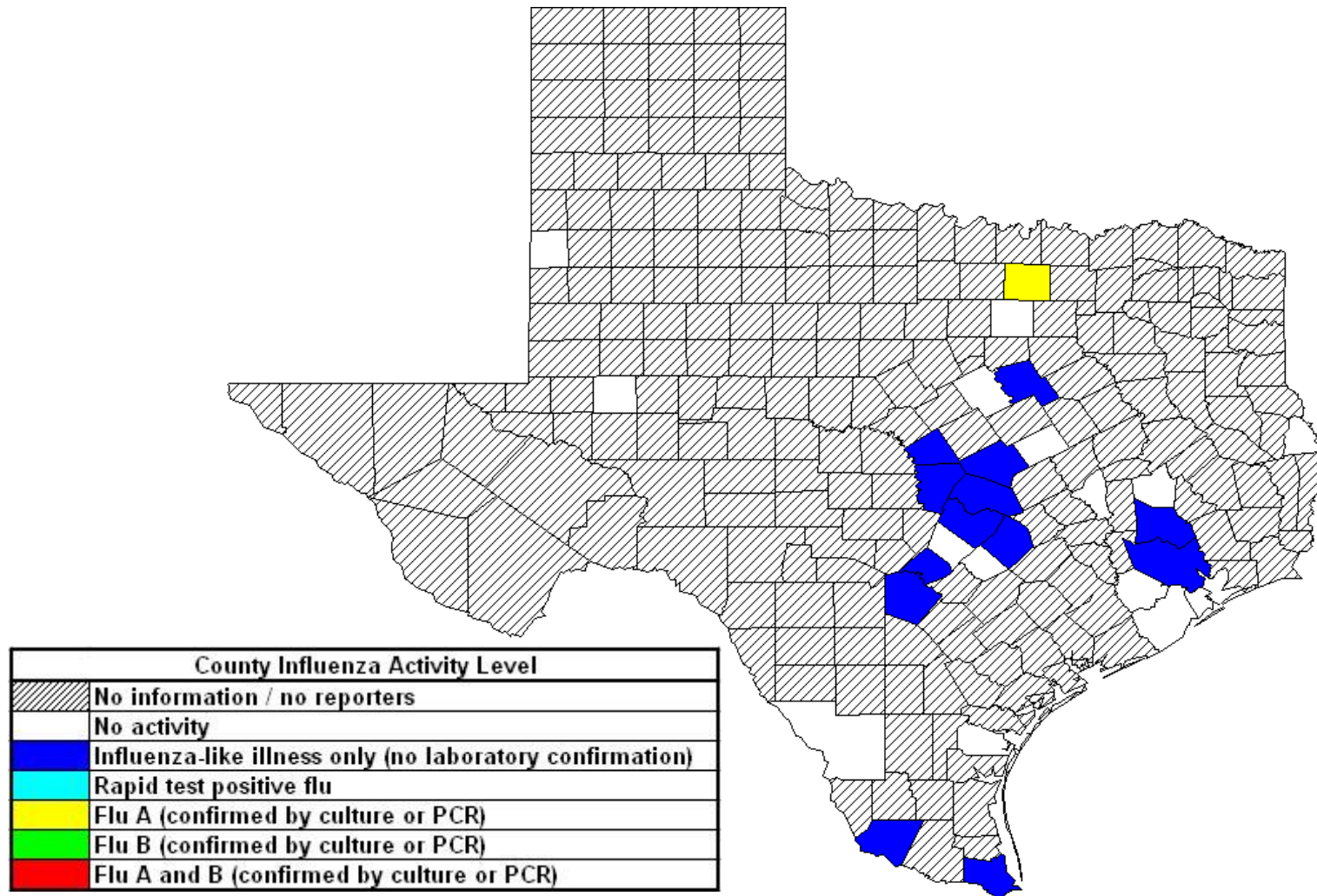
Figure 2: Texas Map Displaying the Highest Level of Influenza or ILI Activity Reported by County for the Week Ending August 15, 2020 (MMWR Week 33)
