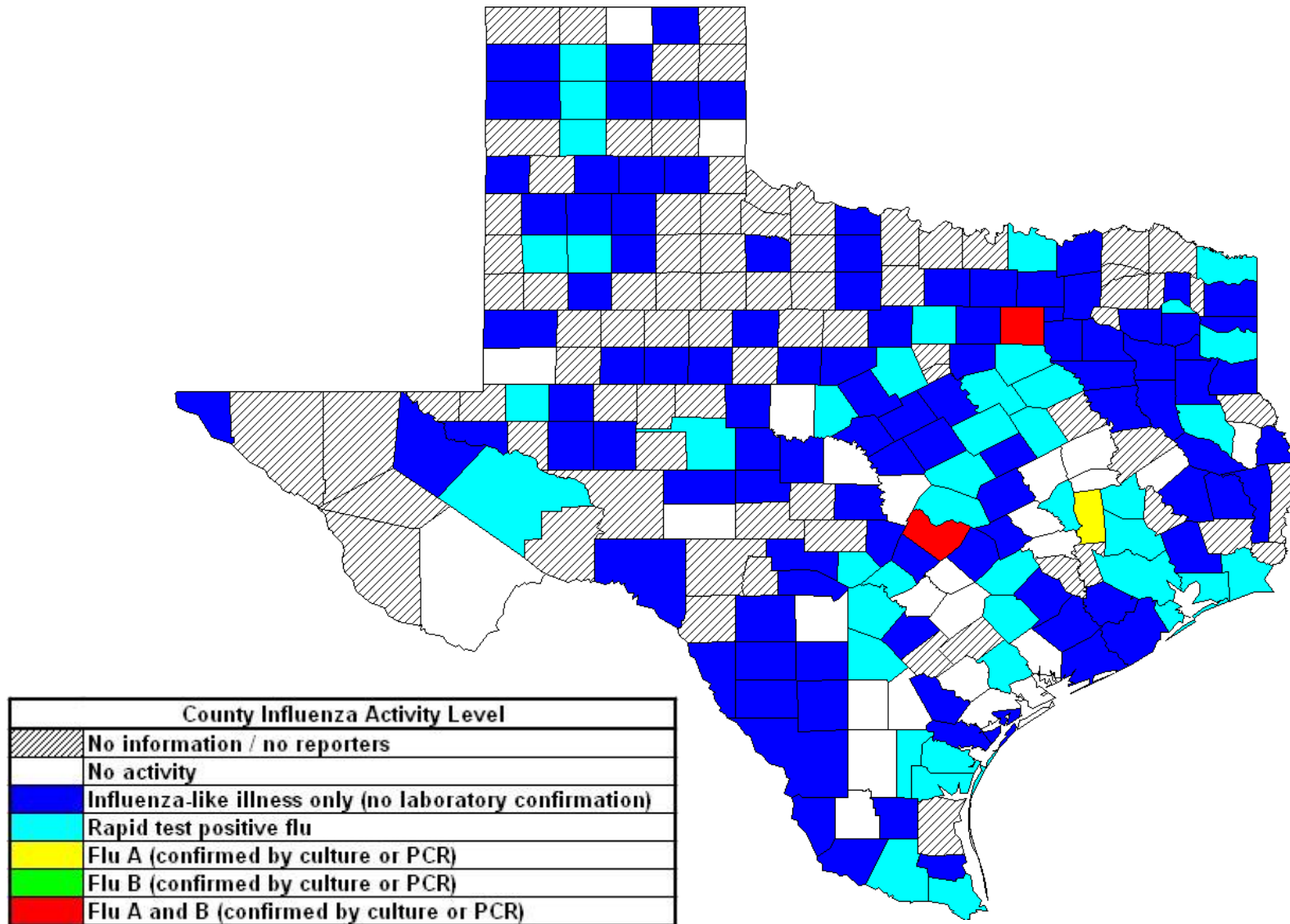
Figure 4: Texas Map Displaying the Highest Level of Influenza or ILI Activity Reported by County for the Week Ending Nov. 14, 2015 (MMWR Week 45)
